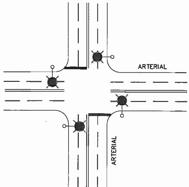
INTERSECTION WITH 4-LANE STREET
