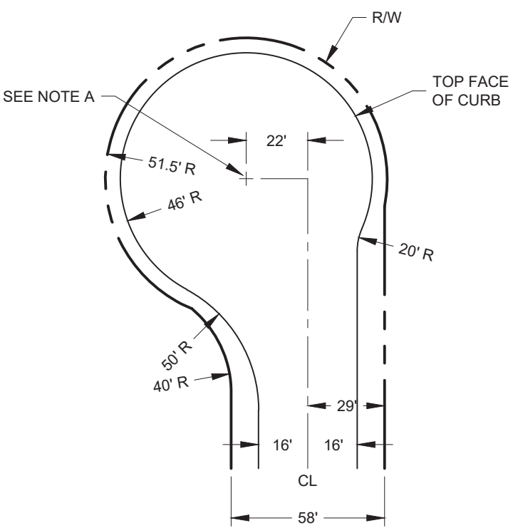
STANDARD CUL-DE-SAC (OFFSET)
