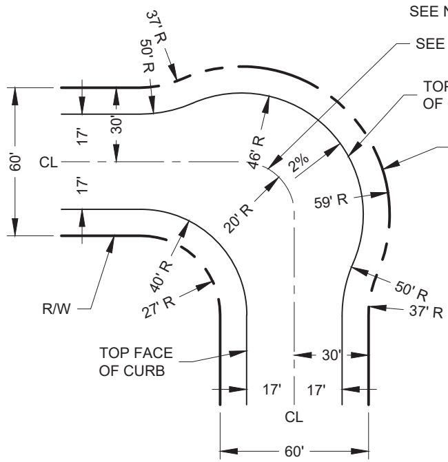
STANDARD EXPANDED CORNER
