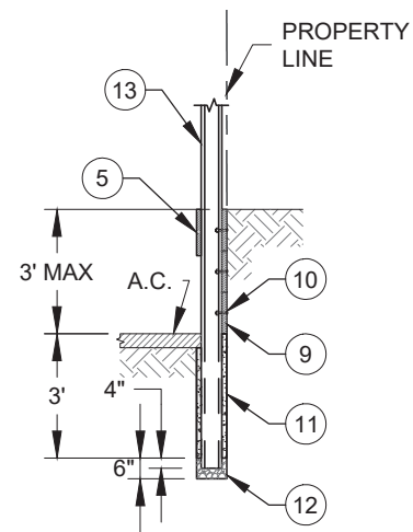
BARRICADE WITH RETAINING WALL RIGHT SIDE VIEW
