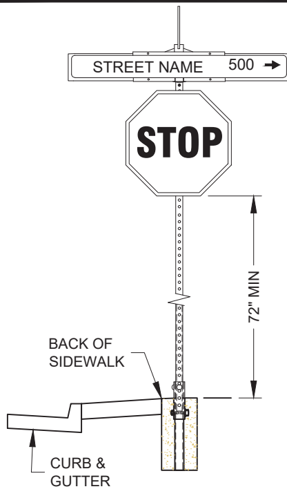
PLACEMENT OF SIGN BEHIND SIDEWALK
