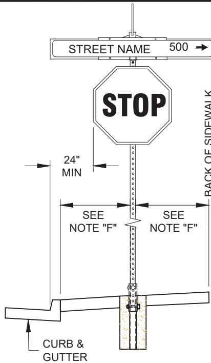
PLACEMENT OF SIGN WITHIN SIDEWALK
