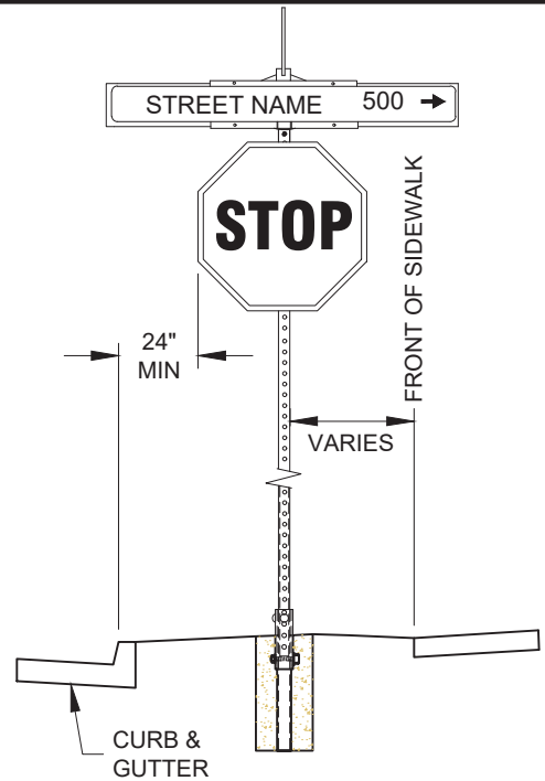
PLACEMENT OF SIGN W/ SEPARATED SIDEWALK
