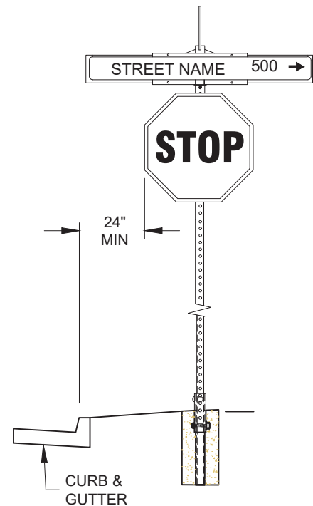
PLACEMENT OF SIGN BEHIND CURB W/O SIDEWALK
