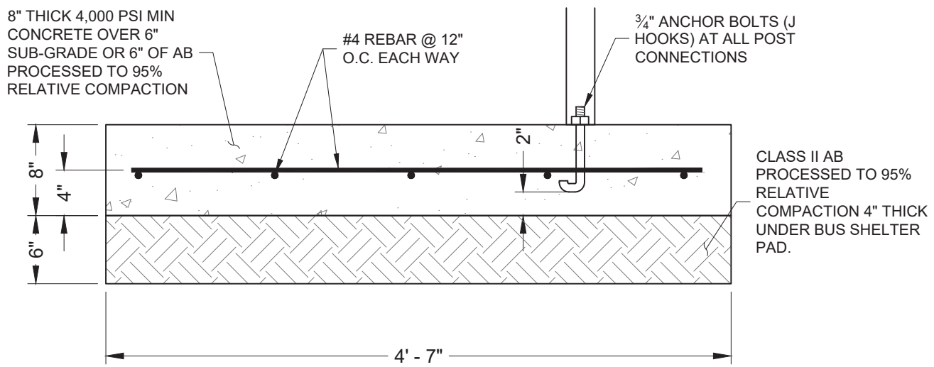
BUS SHELTER FOUNDATION DETAIL
