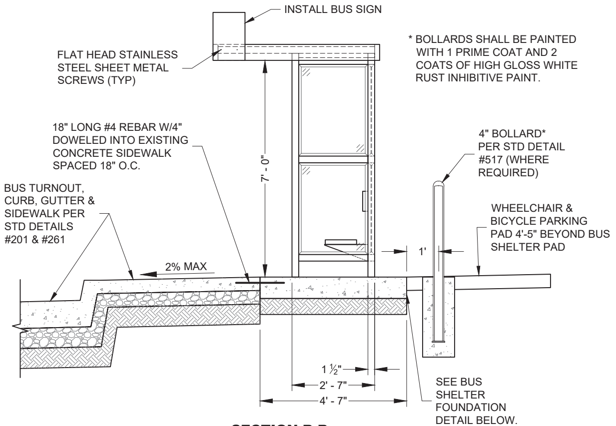
SECTION B-B
