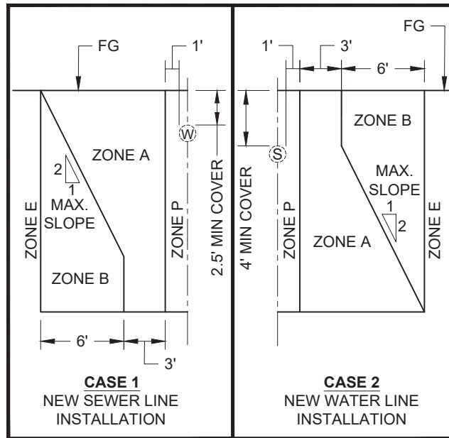
PARALLEL UNDERGROUND INSTALLATION ZONES ½ SECTION VIEWS
